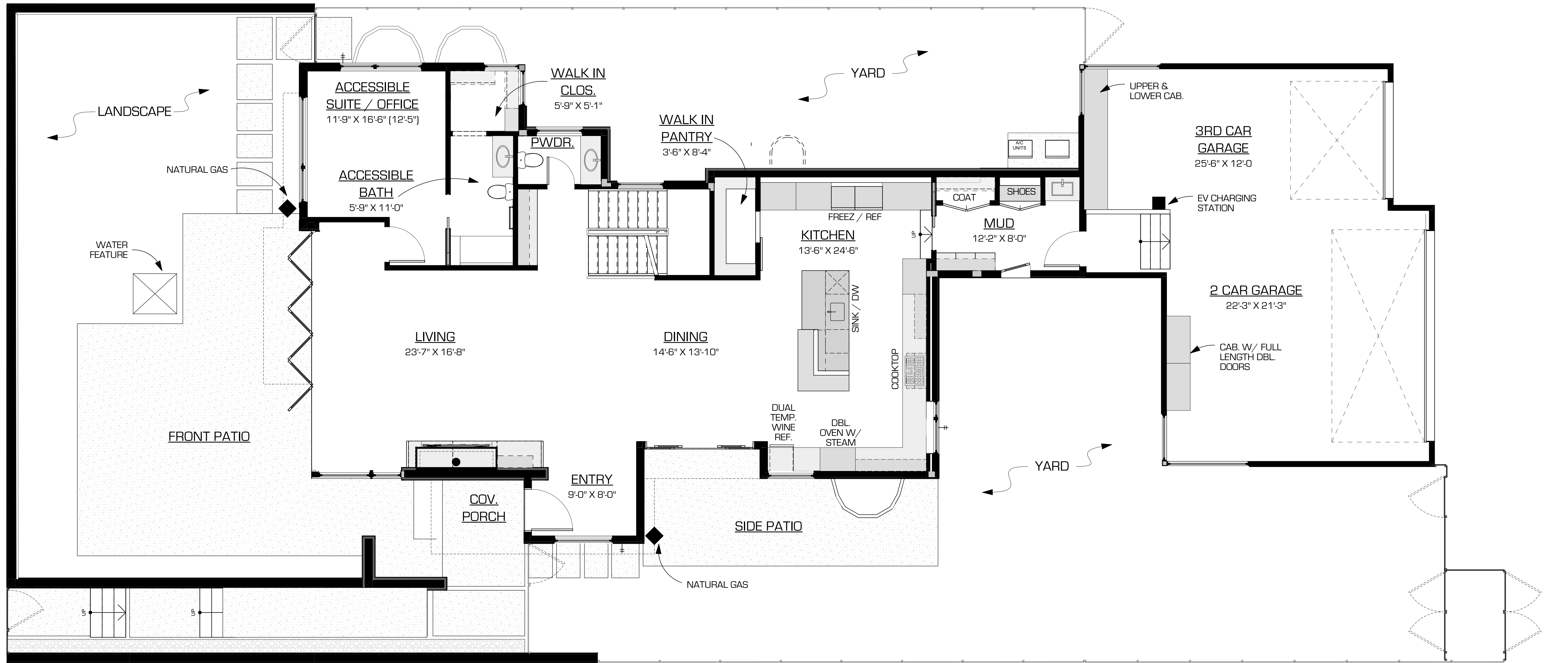
① MAIN LEVEL FLOOR PLAN SCALE: 1/4" = 1'-0"
